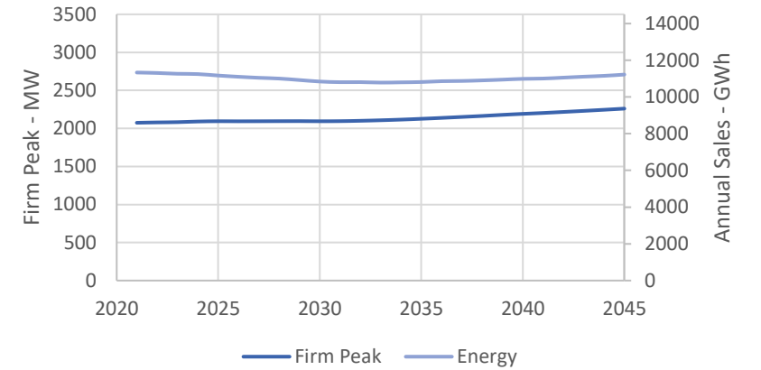
Load Forecast
