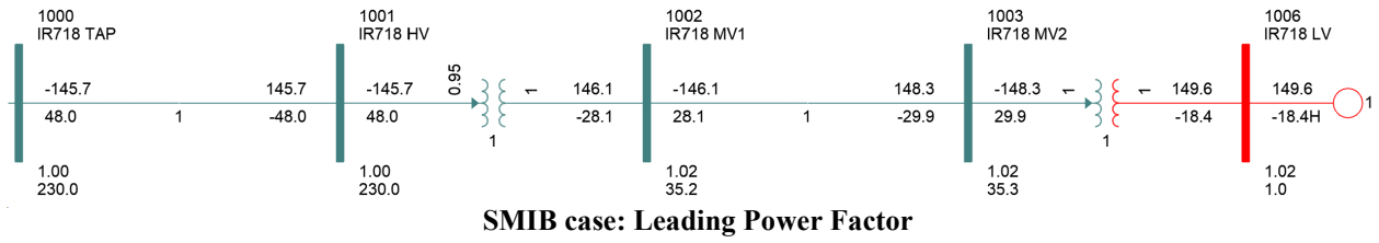
Figure 5: Power Factor Analysis
