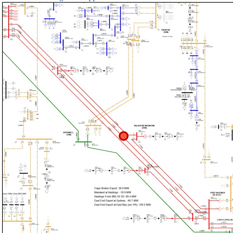
Figure 2: Approximate electrical location of IR#718
