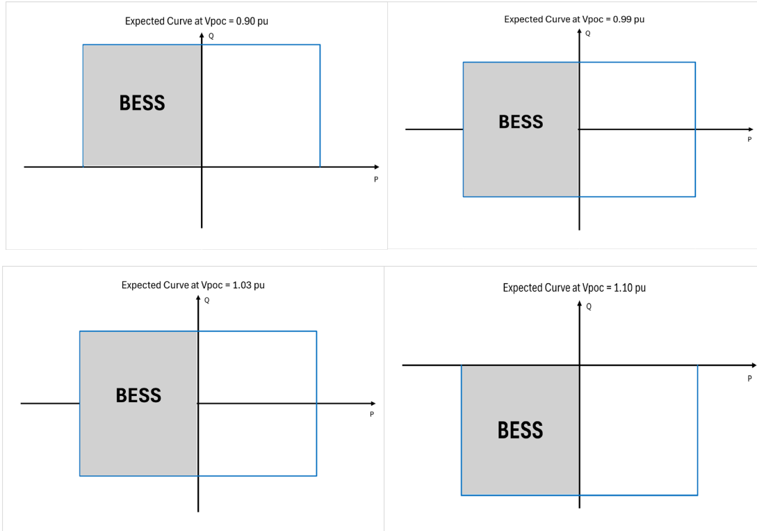
Figure 10: PQ Capability Curves at Different Voltages
