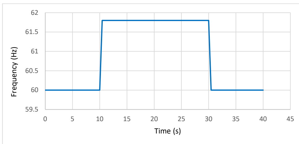
Figure 8: Grid Frequency Change - Over Frequency
