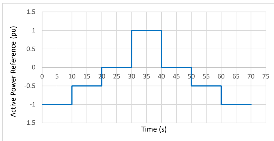
Figure 5: Active Power Reference Change for BESS
