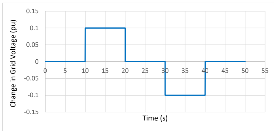
Figure 7: Grid Voltage Change – 2
