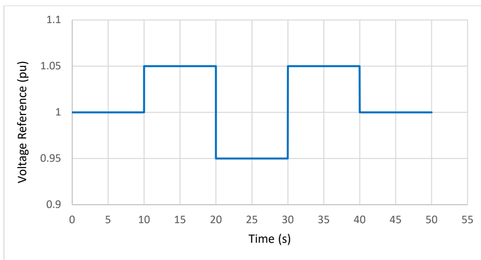
Figure 2: Voltage Reference Change
